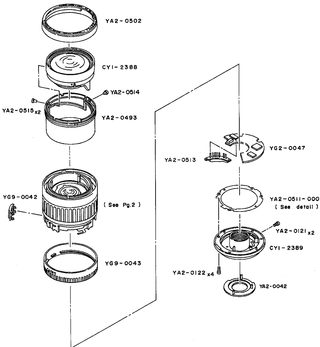
YA2-0511-000 detail
